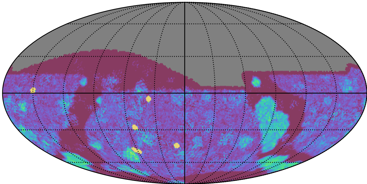
too_elab_heavy_r128_d2_gz_v3.4_10yrs All sky g band: NVisits
