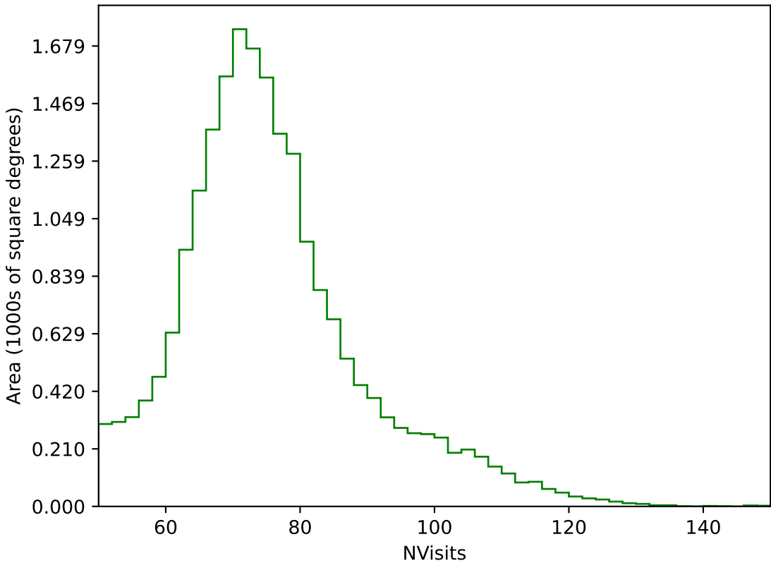
too_elab_heavy_r128_d2_gz_v3.4_10yrs All sky g band: NVisits
