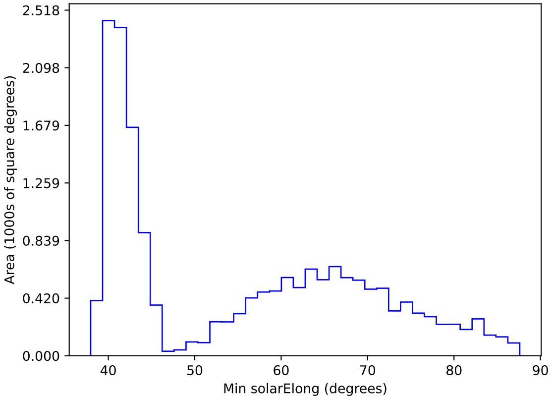
too_elab_heavy_r128_d2_gz_v3.4_10yrs WFD r band: Min solarElong
