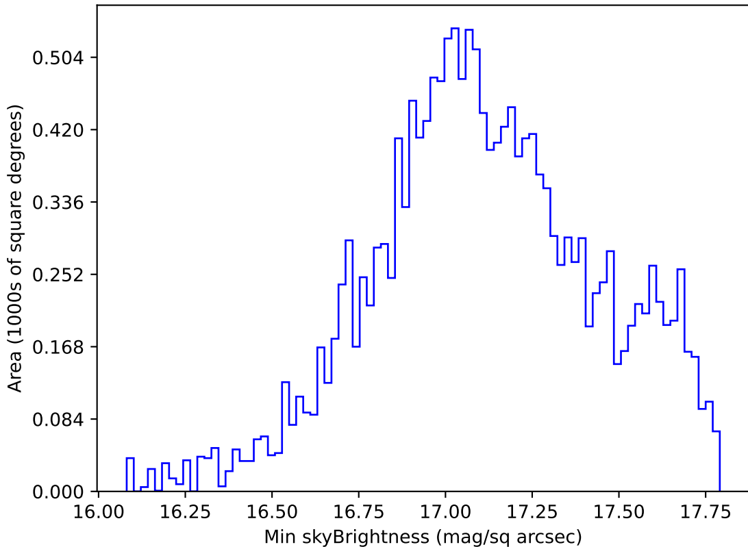
too_elab_heavy_r128_d2_gz_v3.4_10yrs WFD y band: Min skyBrightness
