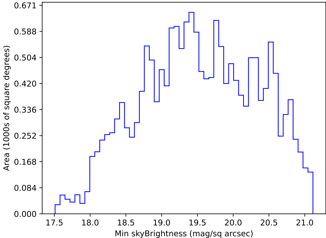
too_elab_heavy_r128_d2_gz_v3.4_10yrs WFD g band: Min skyBrightness
