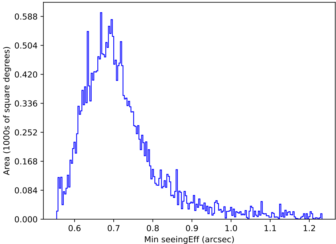
too_elab_heavy_r128_d2_gz_v3.4_10yrs Yr 1 z band: Min seeingEff
