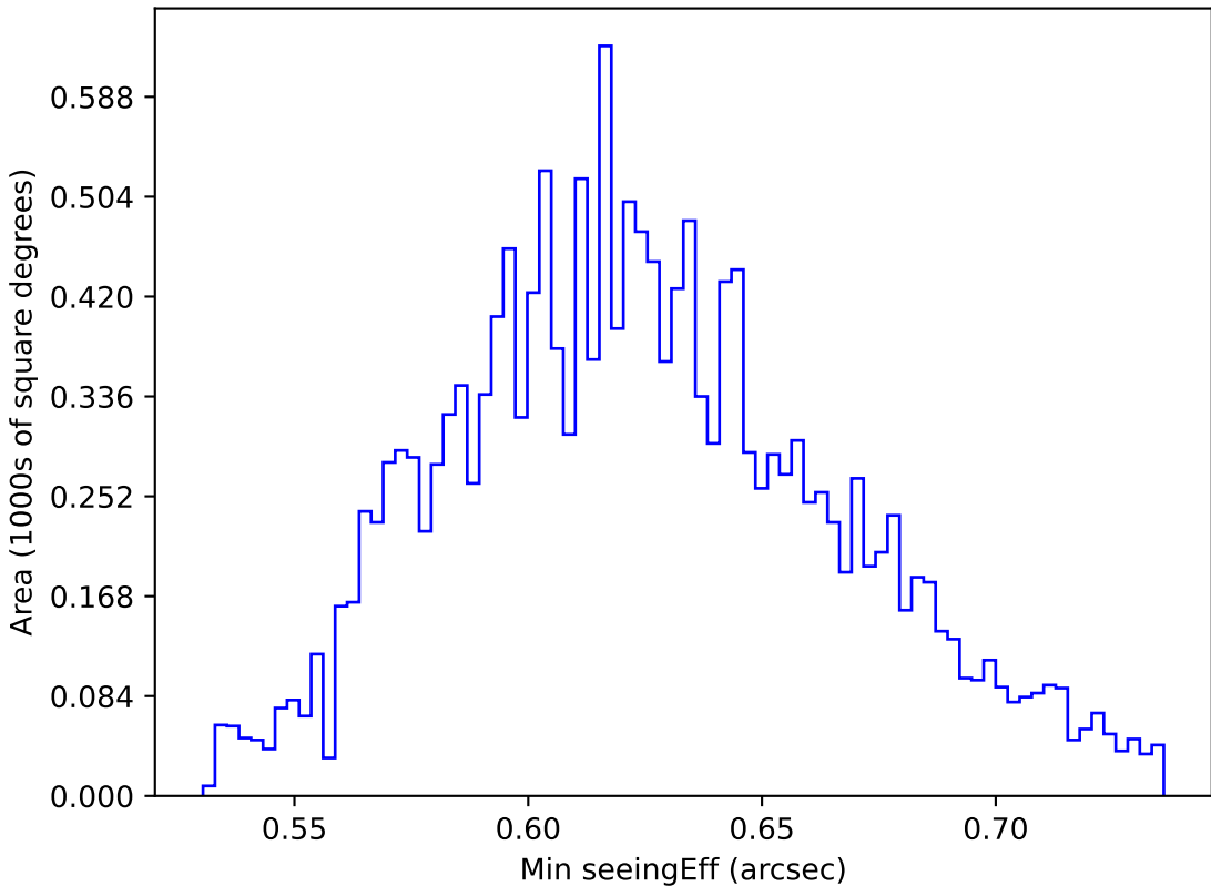
too_elab_heavy_r128_d2_gz_v3.4_10yrs WFD y band: Min seeingEff
