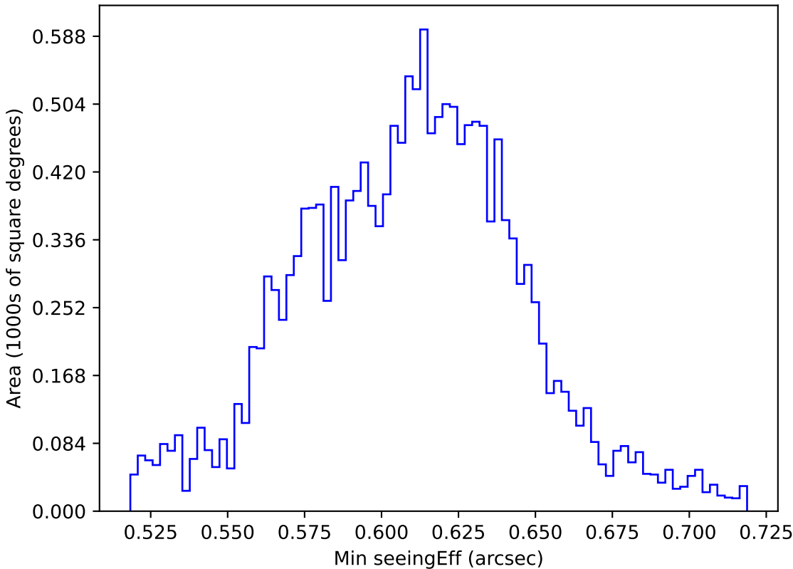
too_elab_heavy_r128_d2_gz_v3.4_10yrs WFD i band: Min seeingEff
