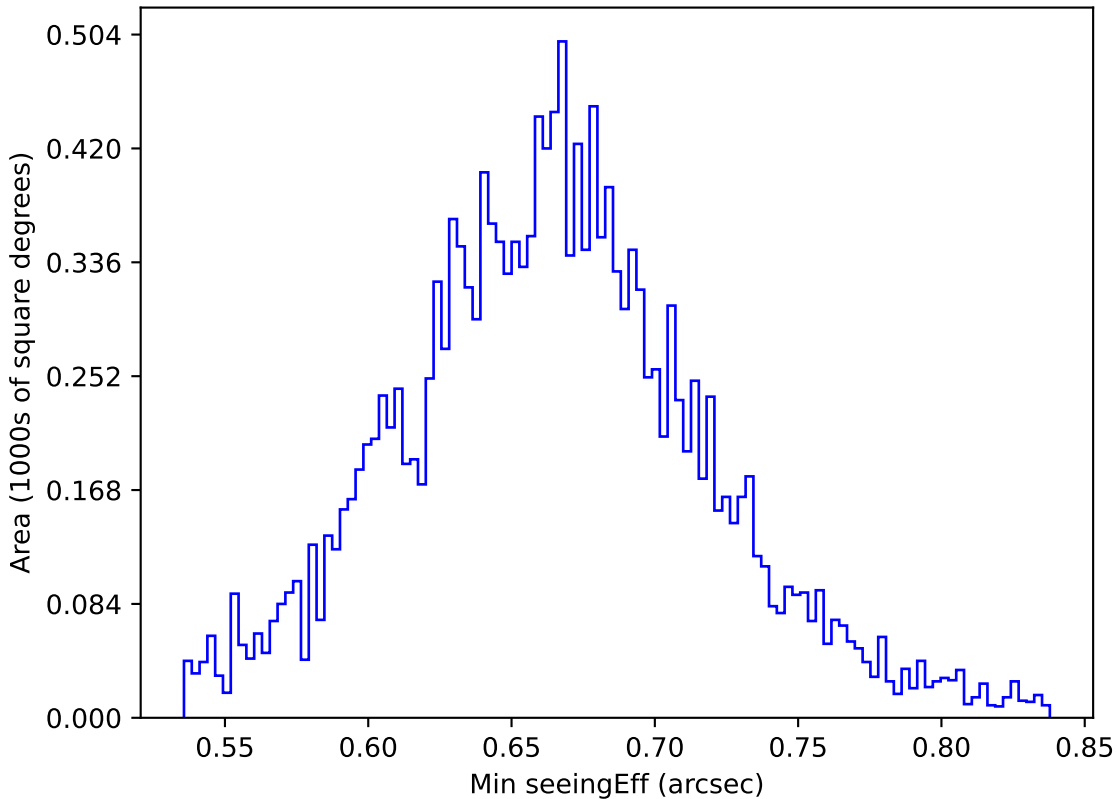
too_elab_heavy_r128_d2_gz_v3.4_10yrs WFD g band: Min seeingEff
