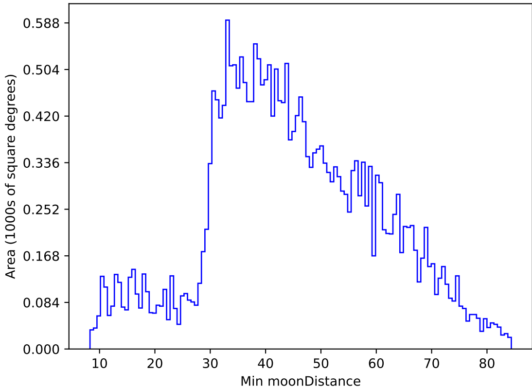
too_elab_heavy_r128_d2_gz_v3.4_10yrs All sky g band: Min moonDistance
