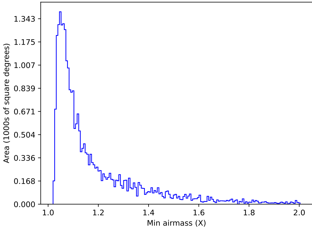
too_elab_heavy_r128_d2_gz_v3.4_10yrs Yr 1 g band: Min airmass
