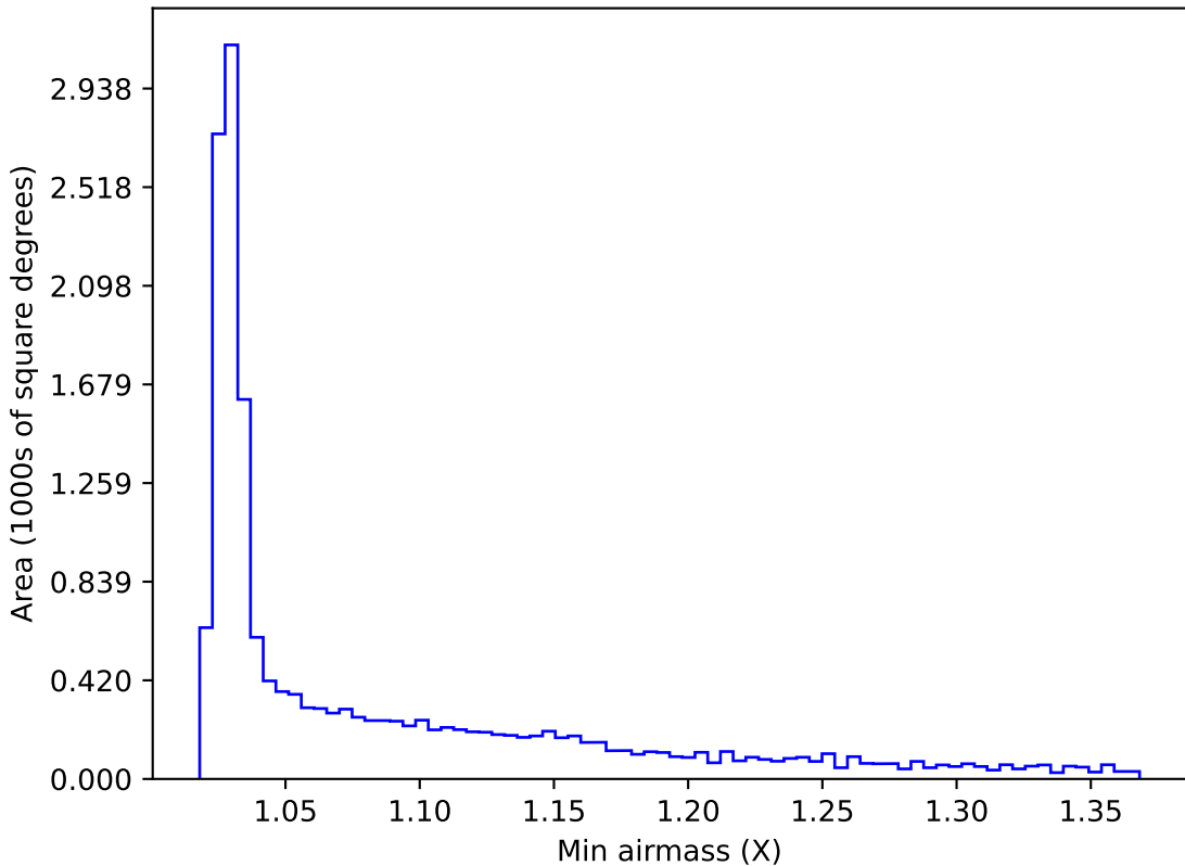
too_elab_heavy_r128_d2_gz_v3.4_10yrs WFD i band: Min airmass
