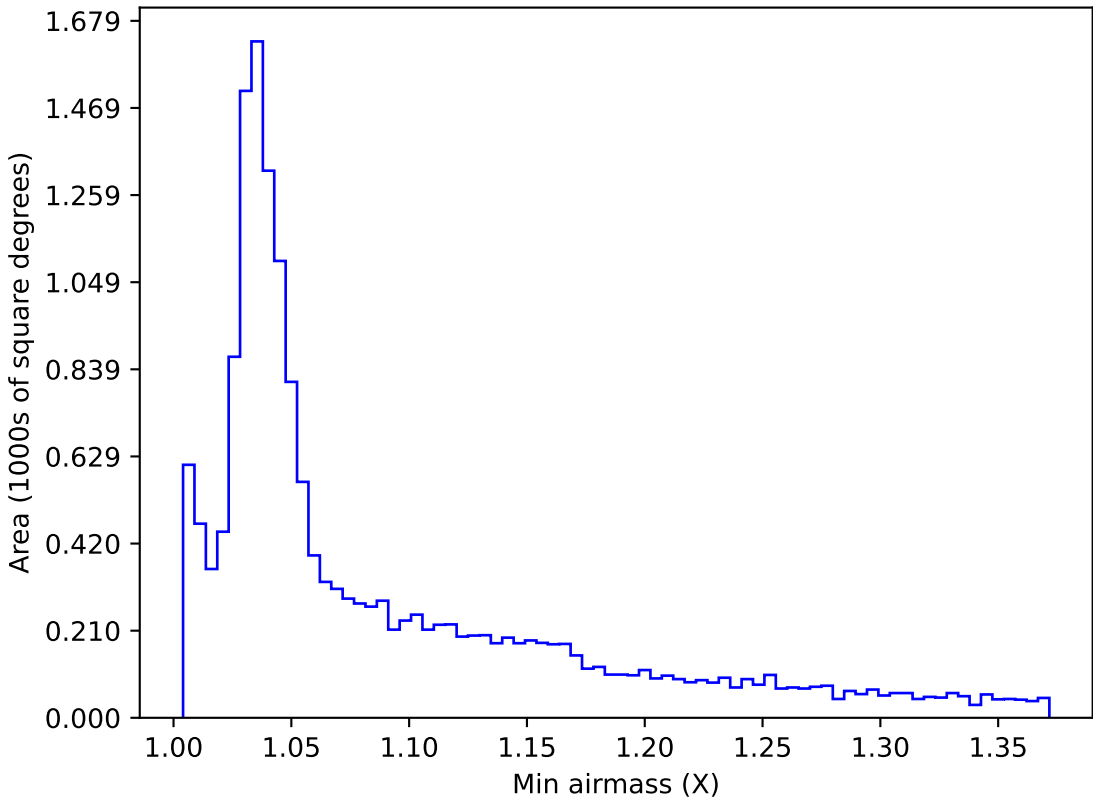
too_elab_heavy_r128_d2_gz_v3.4_10yrs WFD g band: Min airmass
