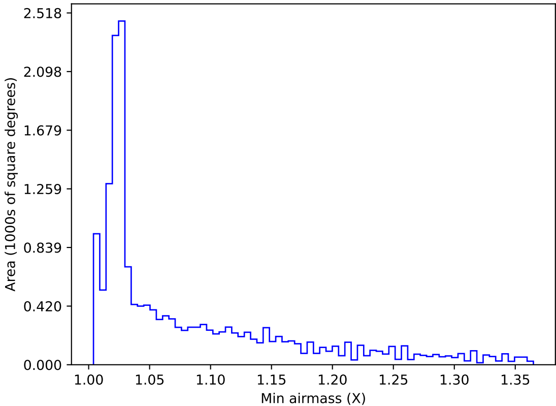
too_elab_heavy_r128_d2_gz_v3.4_10yrs WFD all bands: Min airmass
