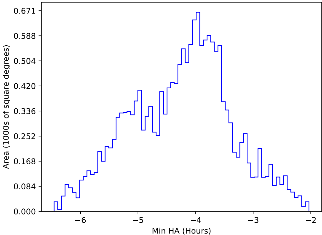
too_elab_heavy_r128_d2_gz_v3.4_10yrs WFD z band: Min HA
