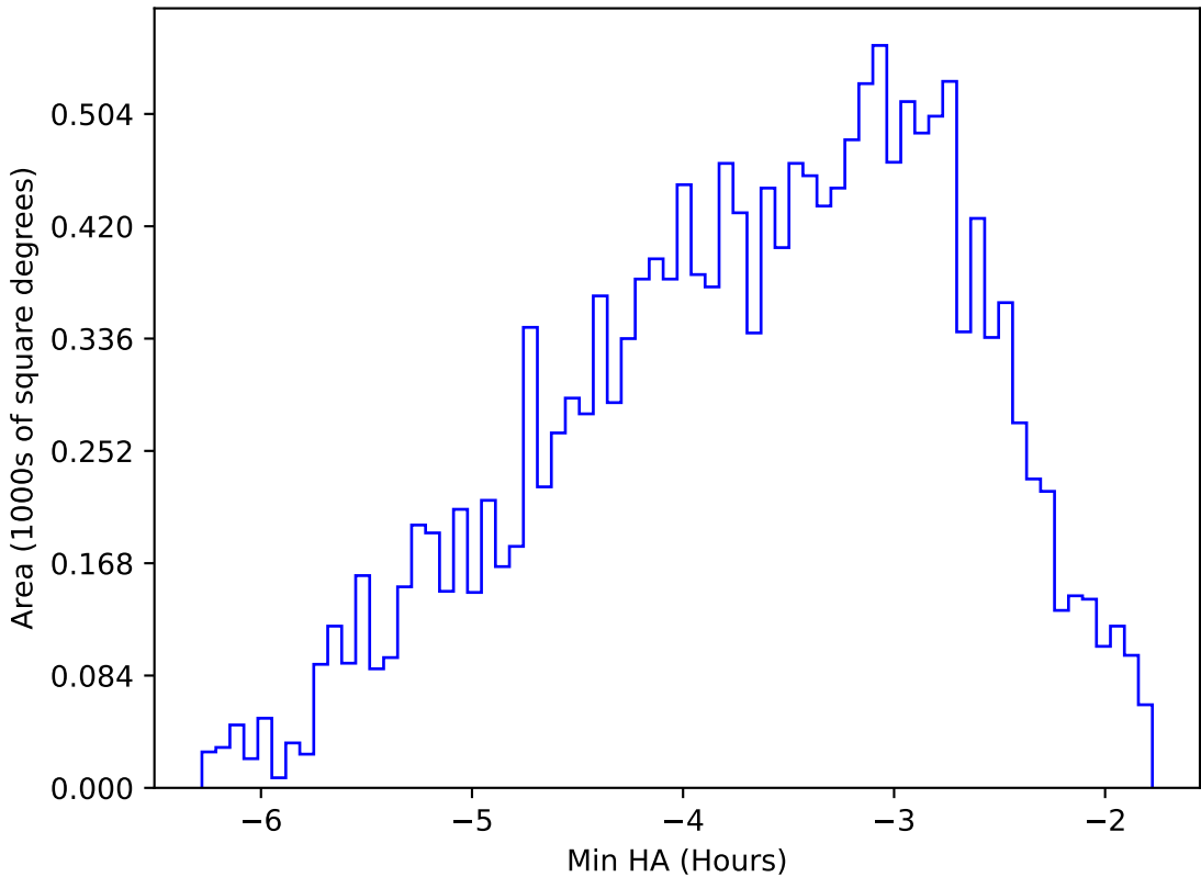
too_elab_heavy_r128_d2_gz_v3.4_10yrs WFD y band: Min HA
