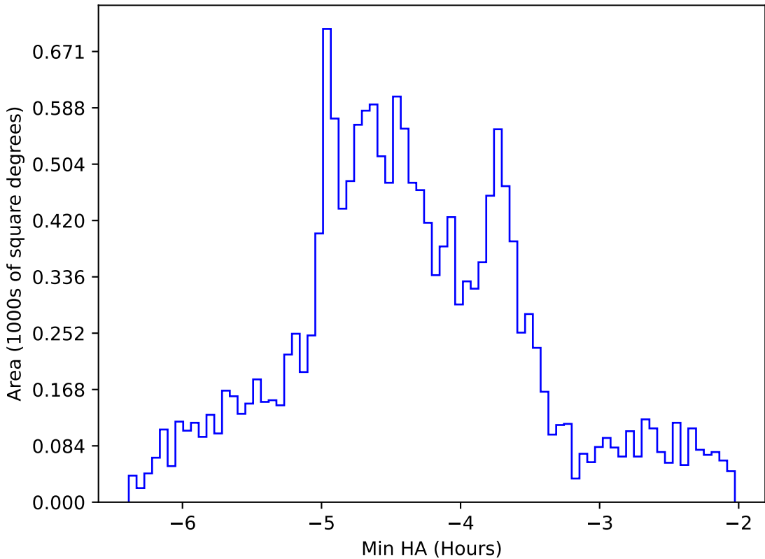
too_elab_heavy_r128_d2_gz_v3.4_10yrs WFD g band: Min HA
