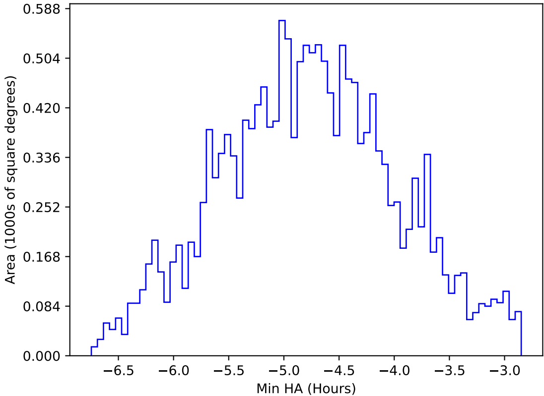
too_elab_heavy_r128_d2_gz_v3.4_10yrs WFD all bands: Min HA
