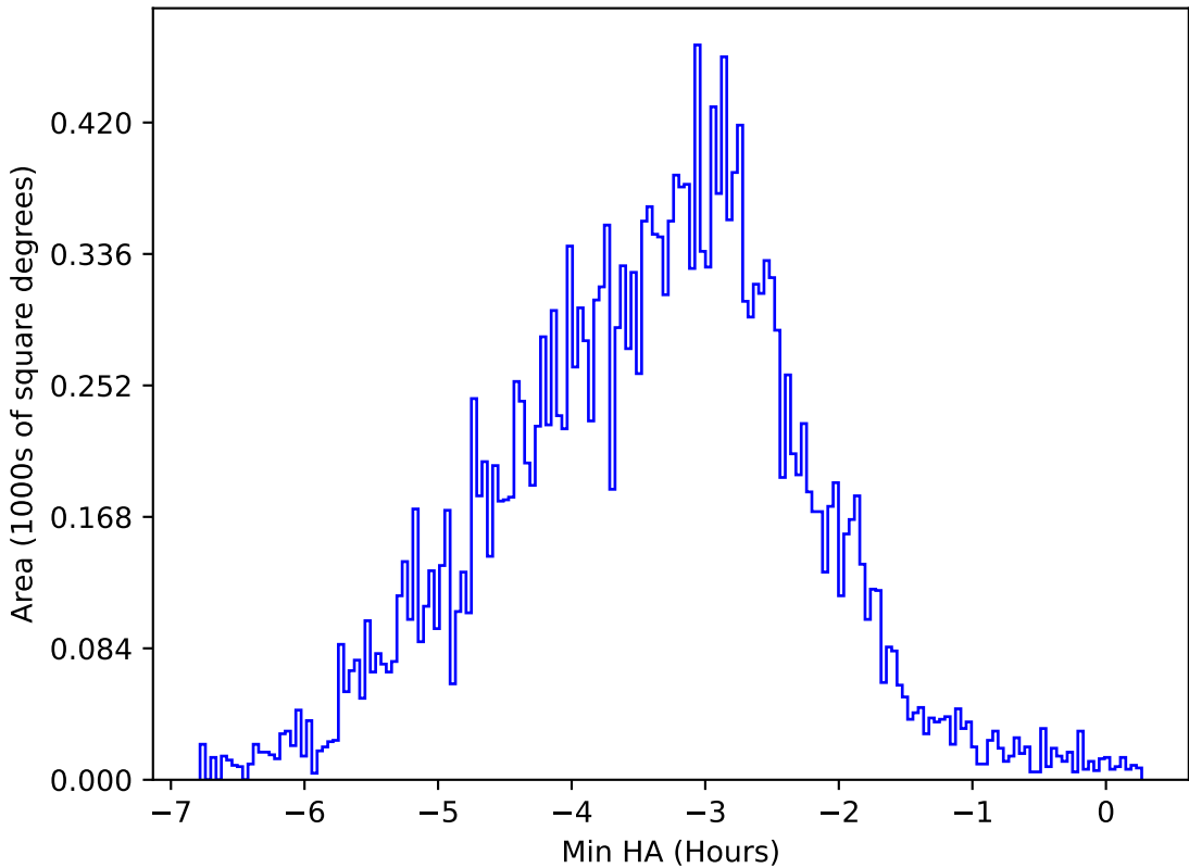
too_elab_heavy_r128_d2_gz_v3.4_10yrs All sky y band: Min HA
