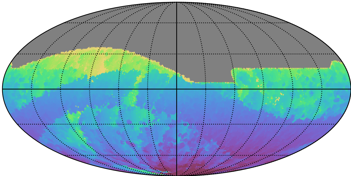
too_elab_heavy_r128_d2_gz_v3.4_10yrs All sky r band: Min HA
