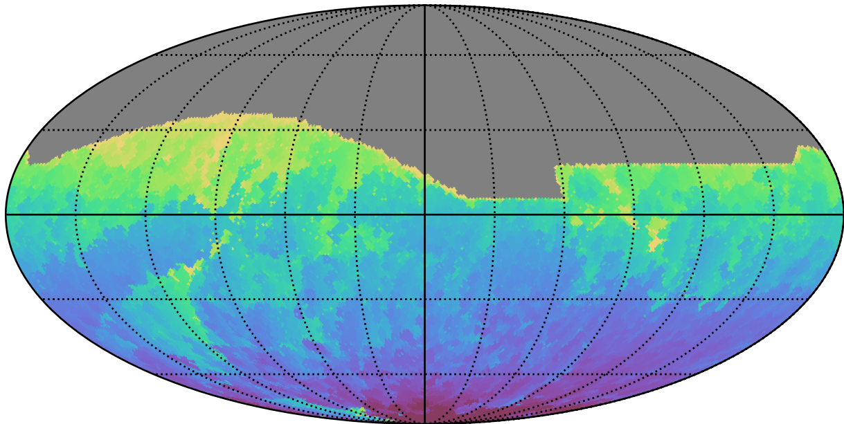
too_elab_heavy_r128_d2_gz_v3.4_10yrs All sky i band: Min HA
