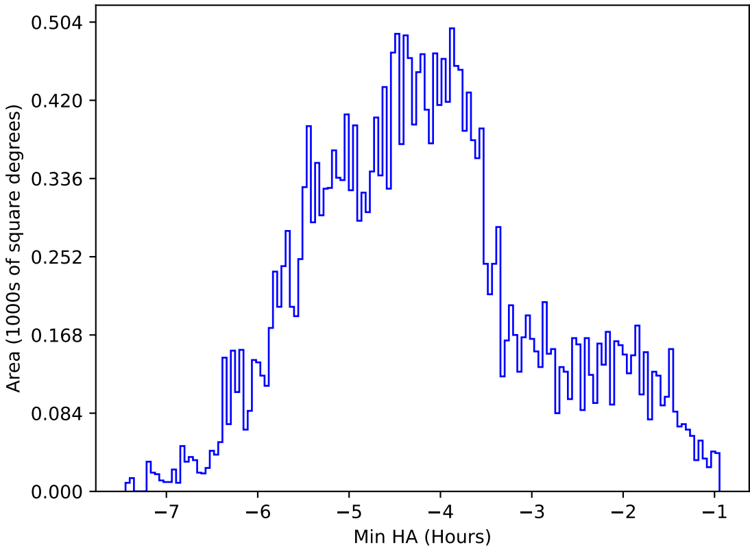
too_elab_heavy_r128_d2_gz_v3.4_10yrs All sky i band: Min HA
