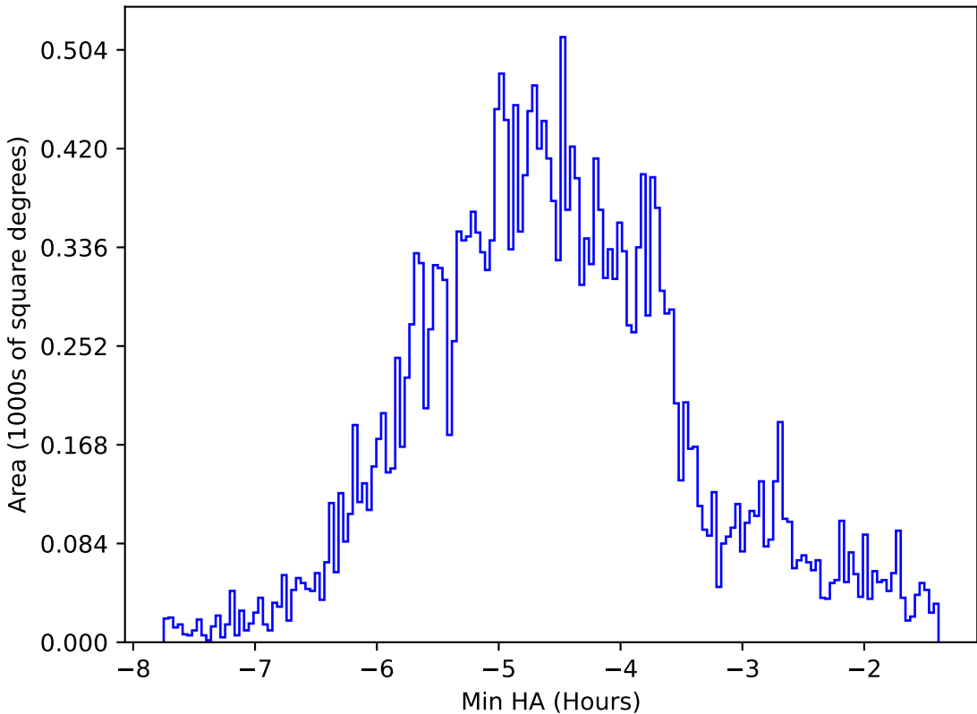
too_elab_heavy_r128_d2_gz_v3.4_10yrs All sky all bands: Min HA
