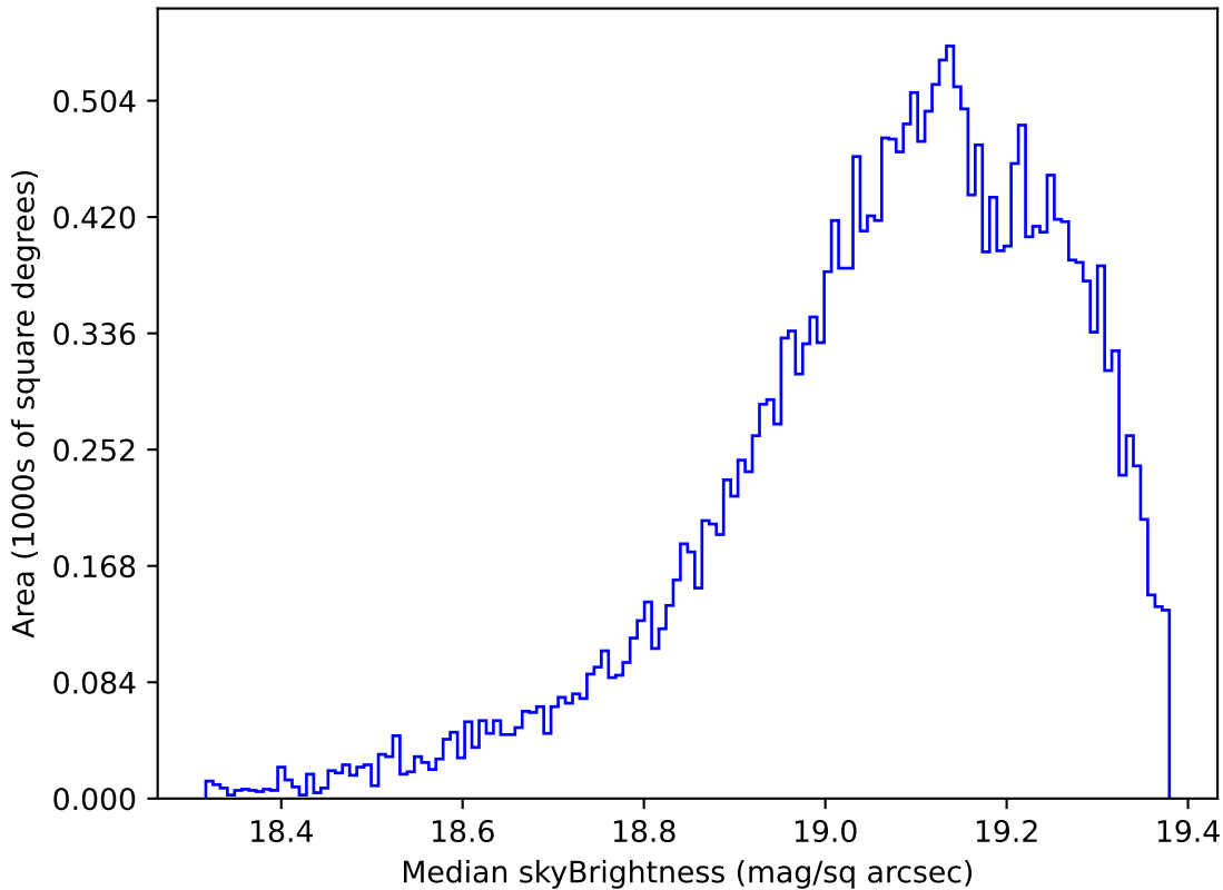
too_elab_heavy_r128_d2_gz_v3.4_10yrs Yr 1 z band: Median skyBrightness
