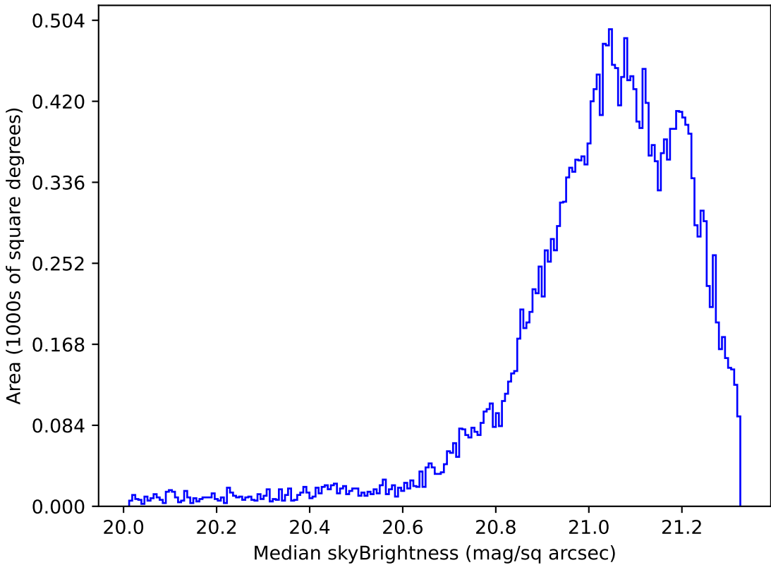
too_elab_heavy_r128_d2_gz_v3.4_10yrs Yr 1 r band: Median skyBrightness
