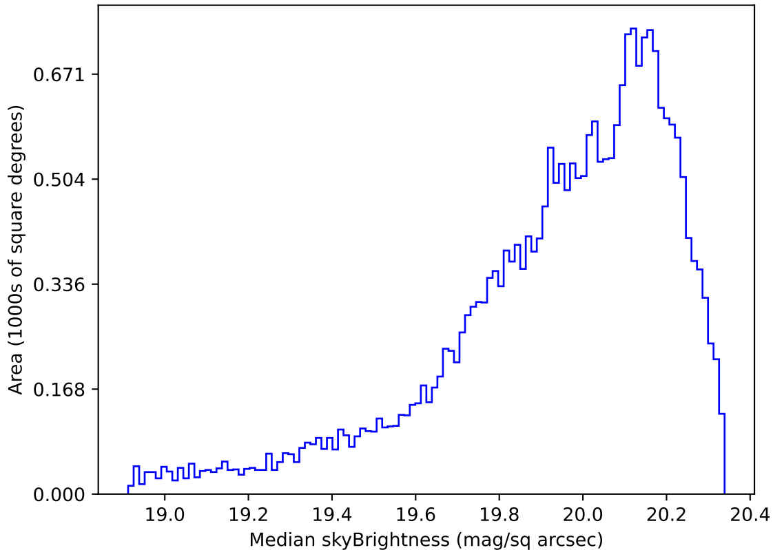
too_elab_heavy_r128_d2_gz_v3.4_10yrs Yr 1 i band: Median skyBrightness
