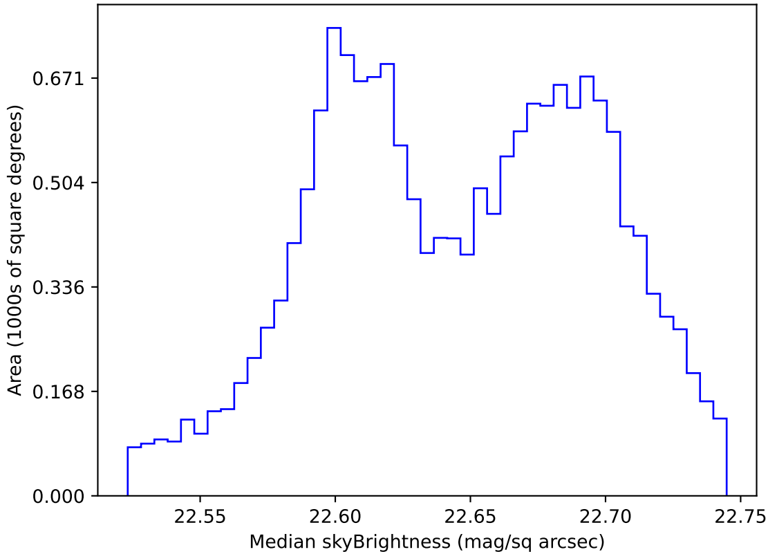
too_elab_heavy_r128_d2_gz_v3.4_10yrs WFD u band: Median skyBrightness
