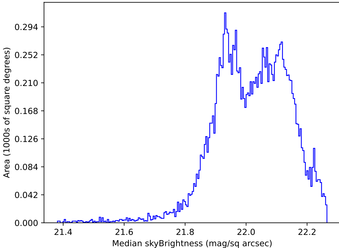
too_elab_heavy_r128_d2_gz_v3.4_10yrs WFD g band: Median skyBrightness
