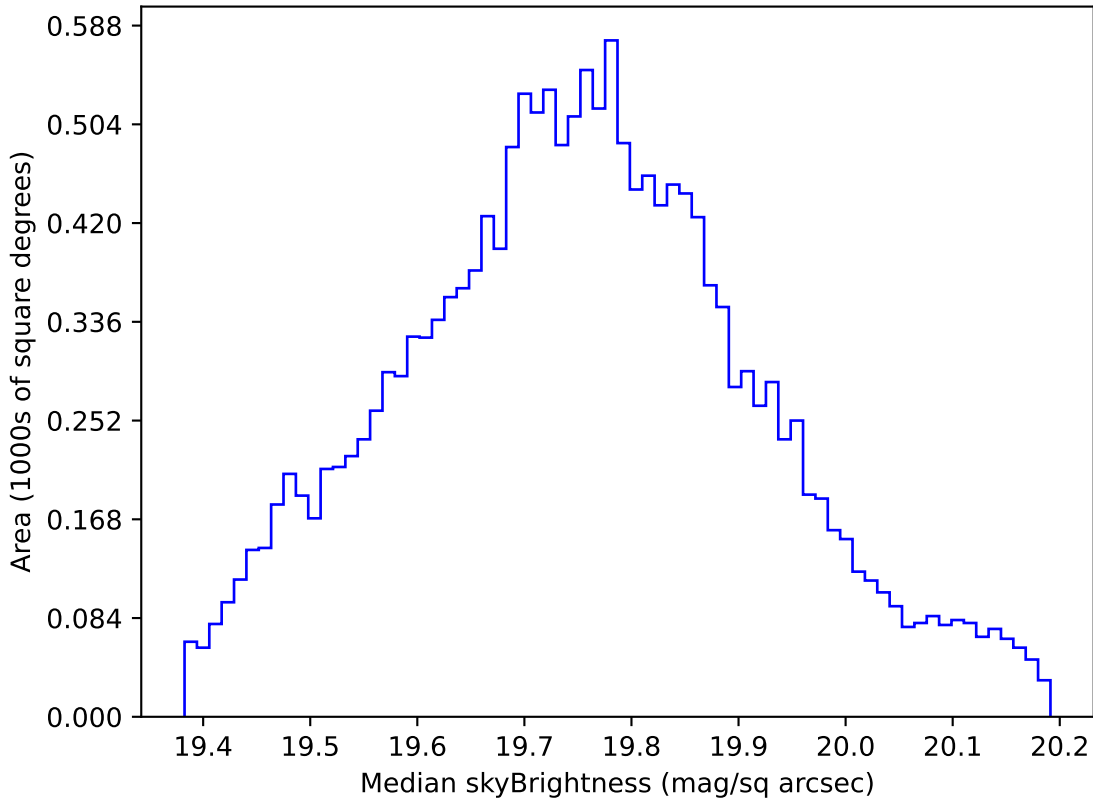
too_elab_heavy_r128_d2_gz_v3.4_10yrs WFD all bands: Median skyBrightness
