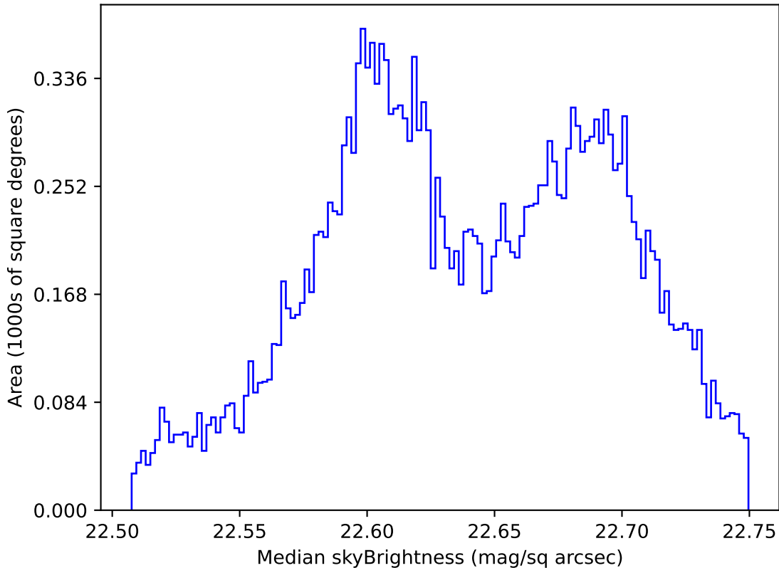
too_elab_heavy_r128_d2_gz_v3.4_10yrs All sky u band: Median skyBrightness
