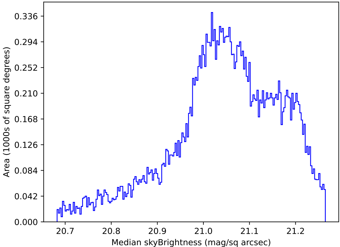
too_elab_heavy_r128_d2_gz_v3.4_10yrs All sky r band: Median skyBrightness
