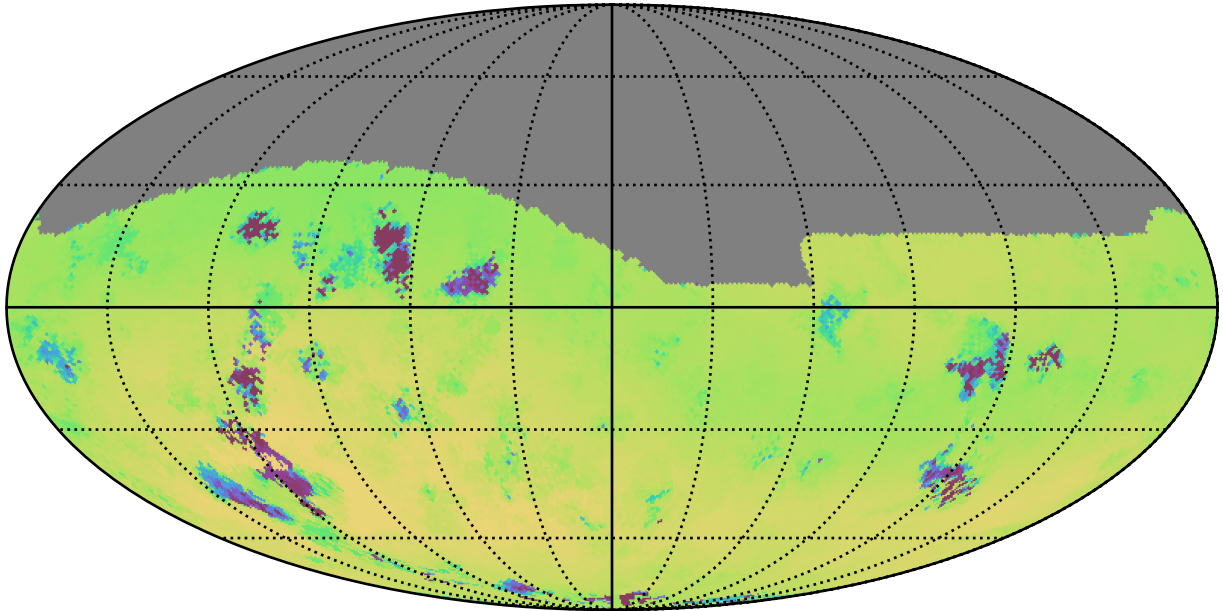
too_elab_heavy_r128_d2_gz_v3.4_10yrs All sky g band: Median skyBrightness
