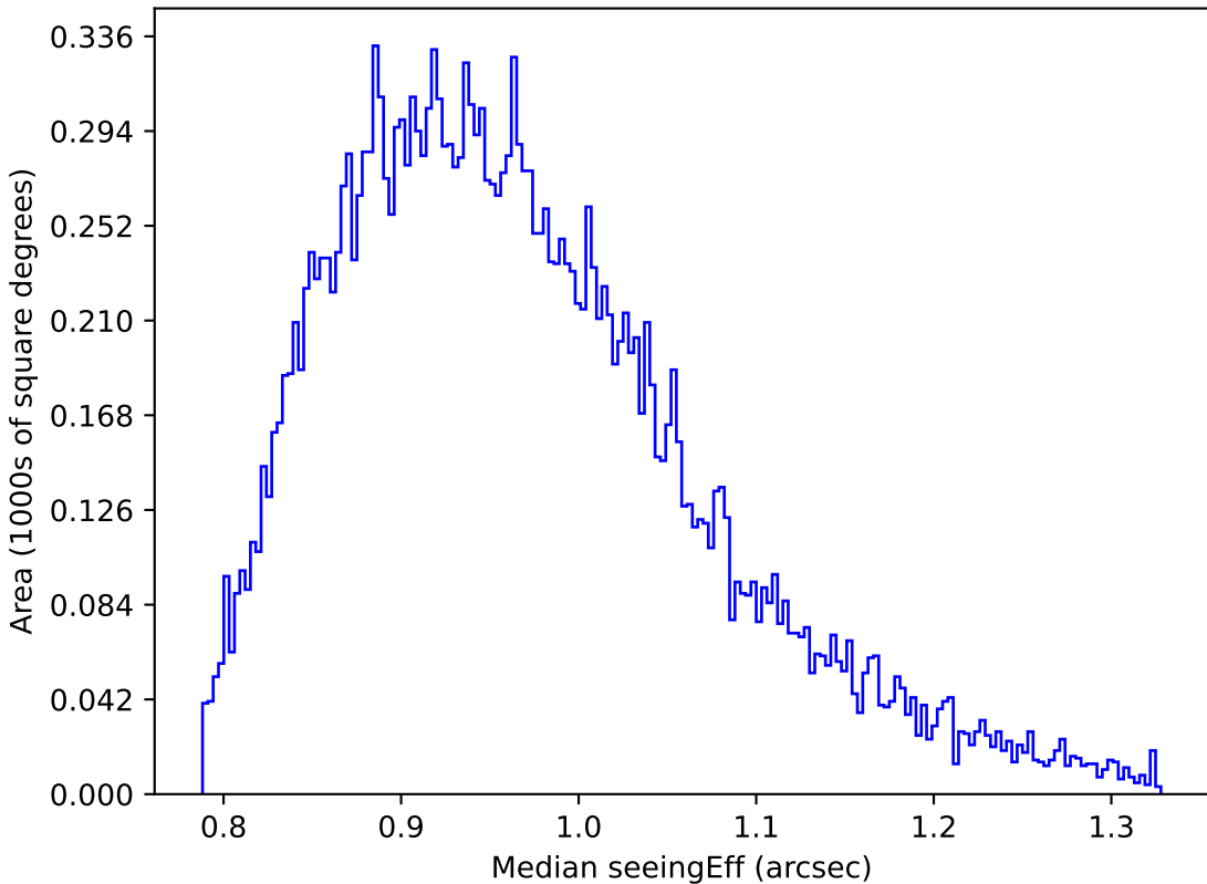
too_elab_heavy_r128_d2_gz_v3.4_10yrs Yr 1 y band: Median seeingEff
