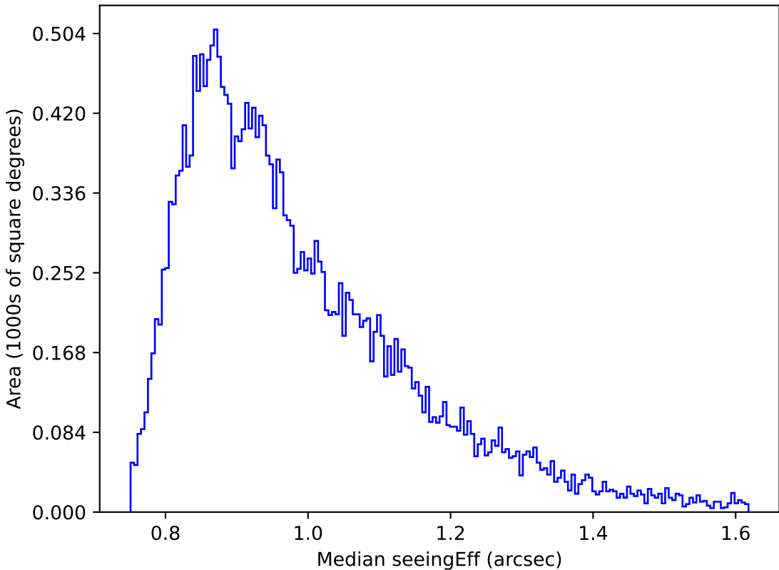
too_elab_heavy_r128_d2_gz_v3.4_10yrs Yr 1 r band: Median seeingEff
