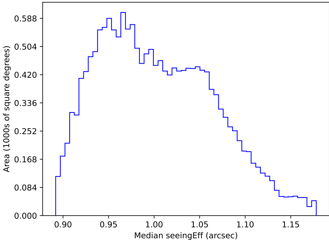
too_elab_heavy_r128_d2_gz_v3.4_10yrs WFD y band: Median seeingEff
