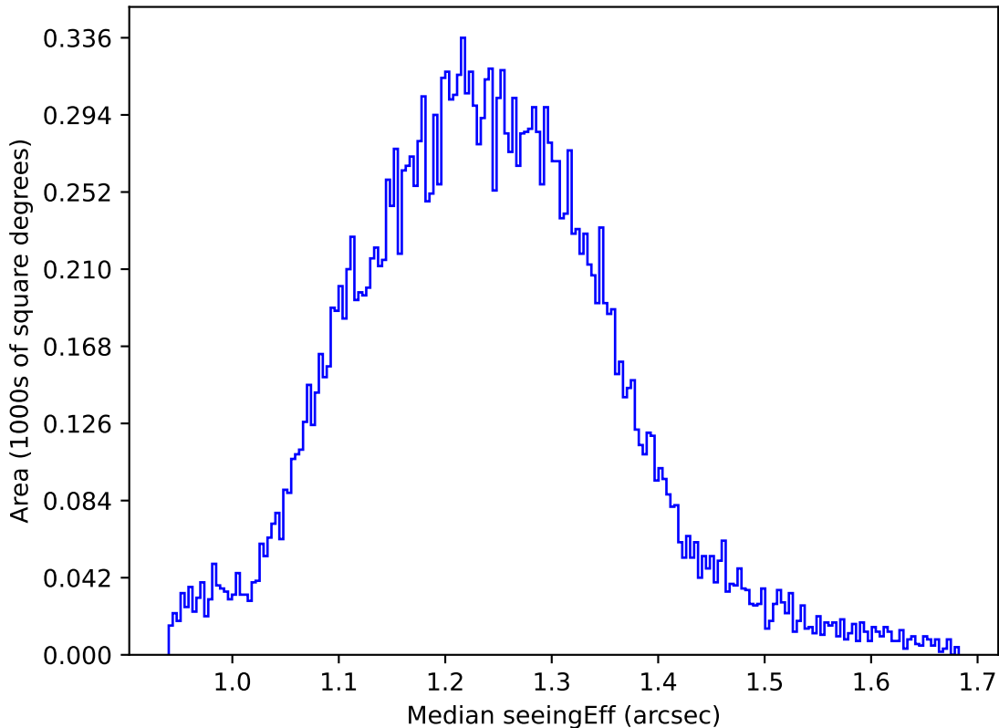
too_elab_heavy_r128_d2_gz_v3.4_10yrs All sky u band: Median seeingEff
