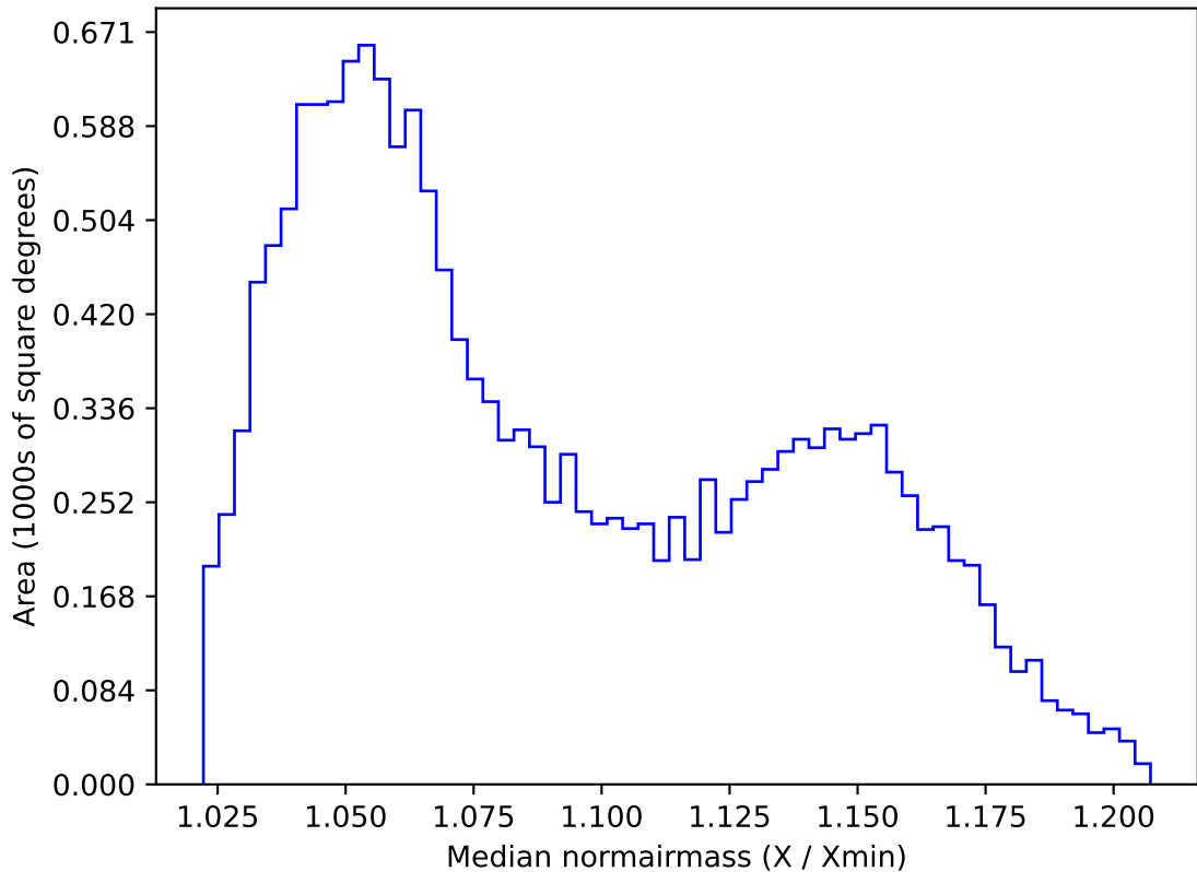
too_elab_heavy_r128_d2_gz_v3.4_10yrs WFD z band: Median normairmass
