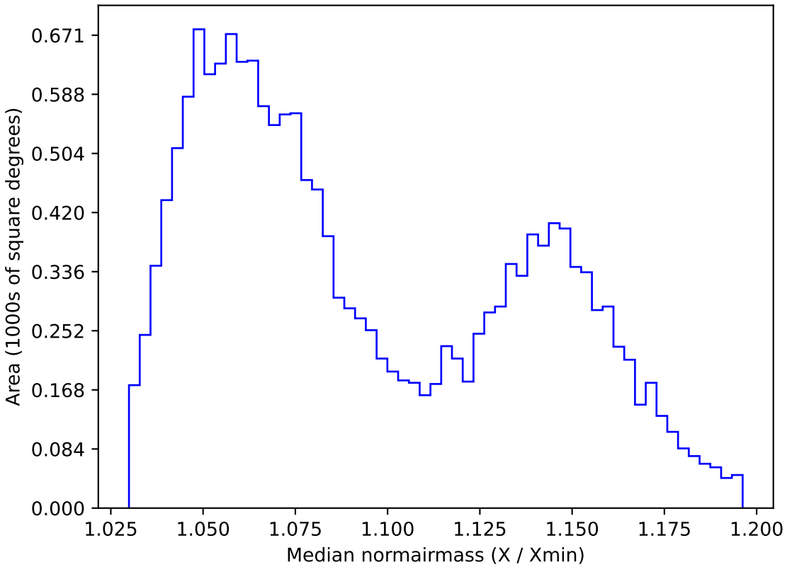
too_elab_heavy_r128_d2_gz_v3.4_10yrs WFD y band: Median normairmass
