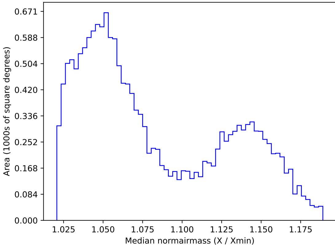
too_elab_heavy_r128_d2_gz_v3.4_10yrs WFD i band: Median normairmass
