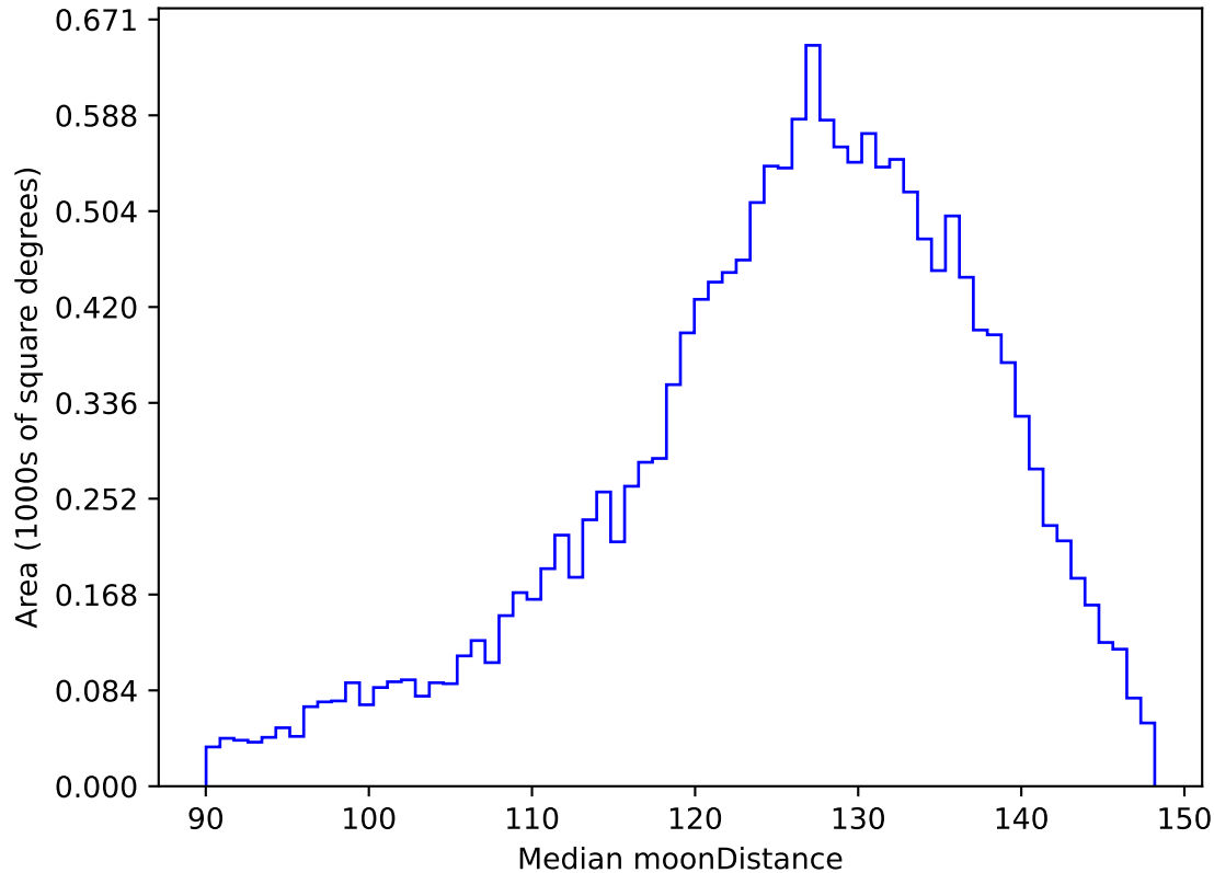
too_elab_heavy_r128_d2_gz_v3.4_10yrs WFD u band: Median moonDistance
