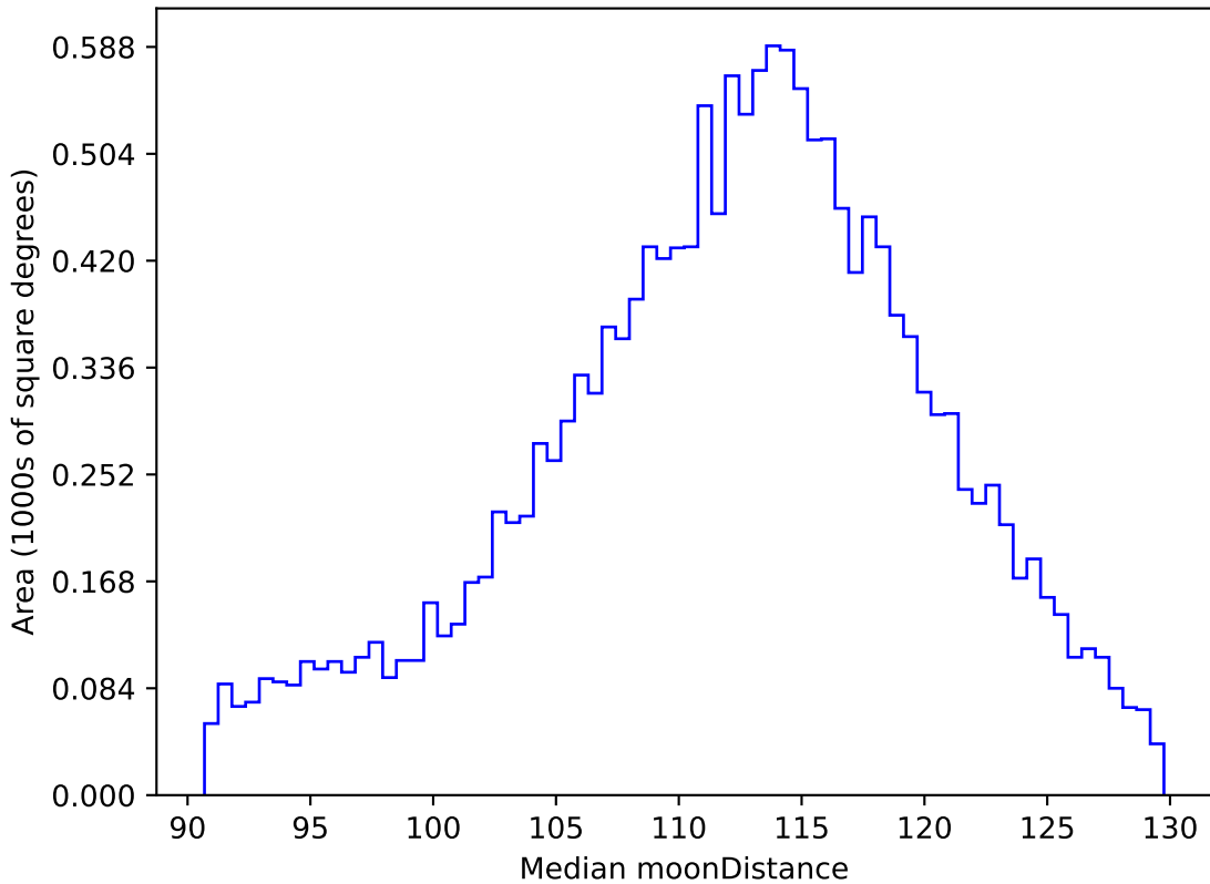
too_elab_heavy_r128_d2_gz_v3.4_10yrs WFD r band: Median moonDistance
