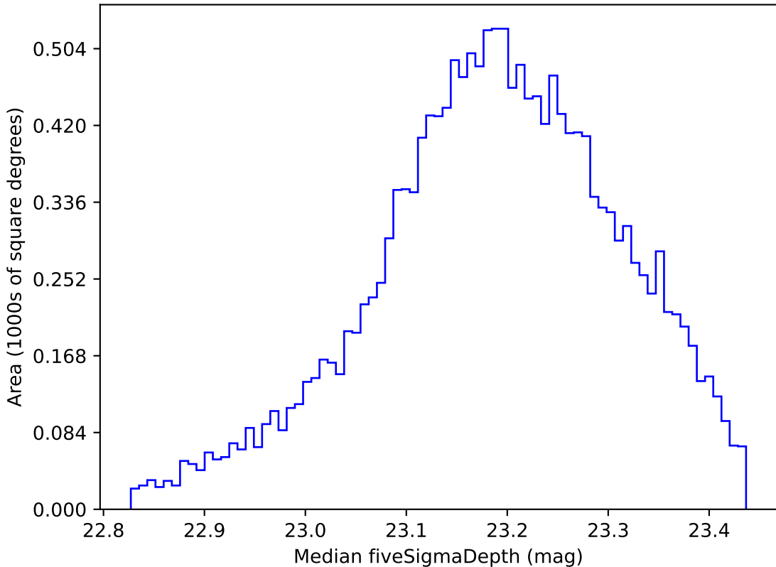
too_elab_heavy_r128_d2_gz_v3.4_10yrs WFD u band: Median fiveSigmaDepth
