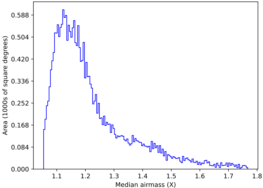
too_elab_heavy_r128_d2_gz_v3.4_10yrs Yr 1 u band: Median airmass
