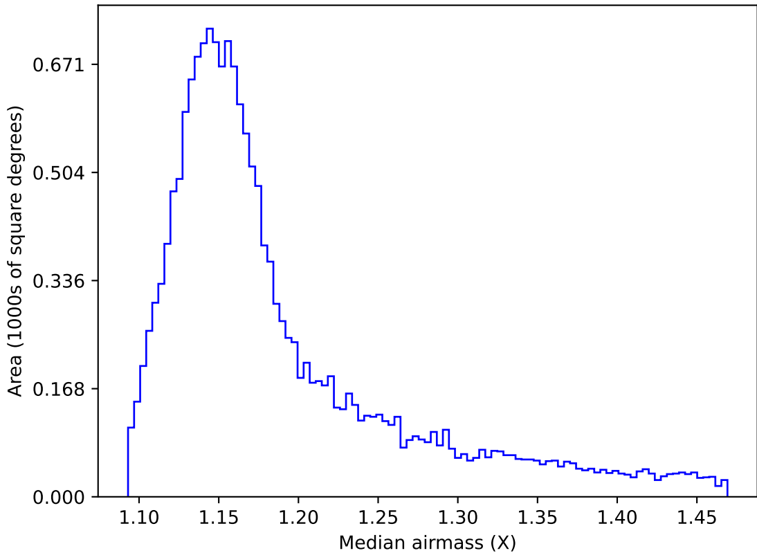
too_elab_heavy_r128_d2_gz_v3.4_10yrs WFD z band: Median airmass
