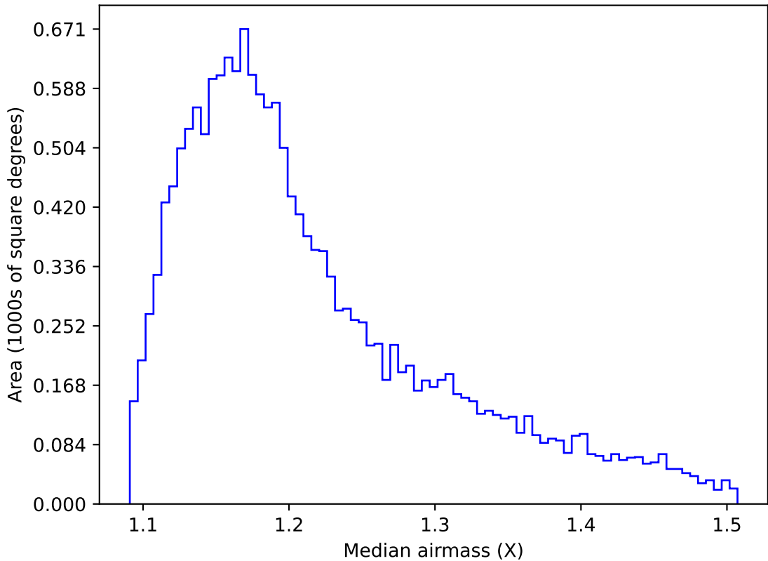
too_elab_heavy_r128_d2_gz_v3.4_10yrs WFD g band: Median airmass
