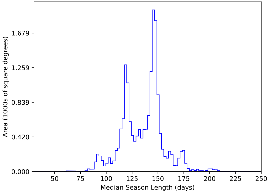
too_elab_heavy_r128_d2_gz_v3.4_10yrs WFD y band: Median Season Length
