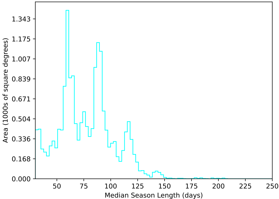
too_elab_heavy_r128_d2_gz_v3.4_10yrs WFD u band: Median Season Length
