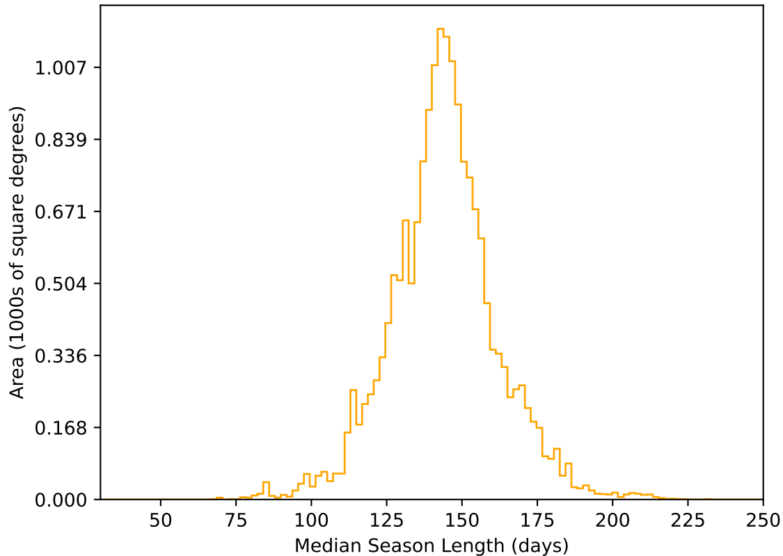
too_elab_heavy_r128_d2_gz_v3.4_10yrs WFD r band: Median Season Length
