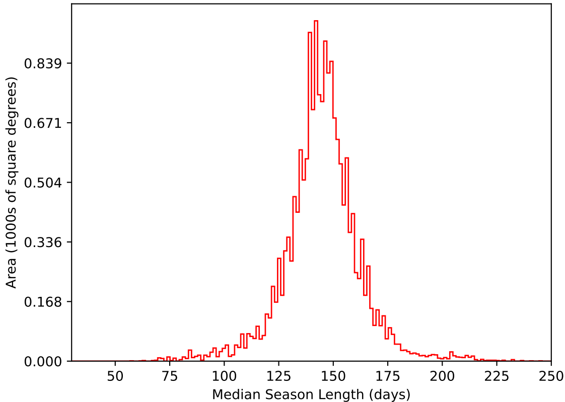
too_elab_heavy_r128_d2_gz_v3.4_10yrs WFD i band: Median Season Length
