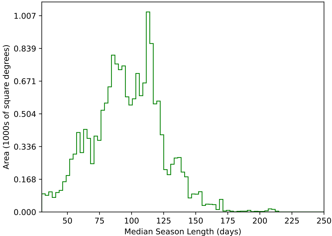
too_elab_heavy_r128_d2_gz_v3.4_10yrs WFD g band: Median Season Length
